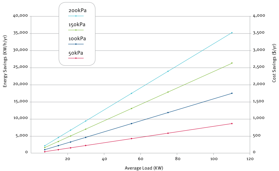
Figure 1: Potential costs and energy savings that can be made by reducing air pressure 2
